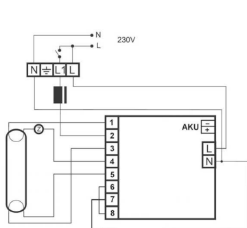
Connection to inductive ballast
