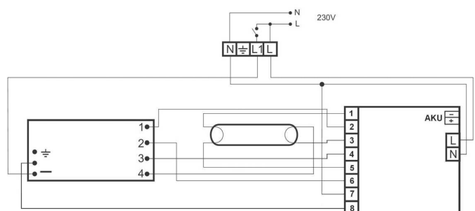
Connection to inductive ballast for fluorescent lamps arranged in serial layout
