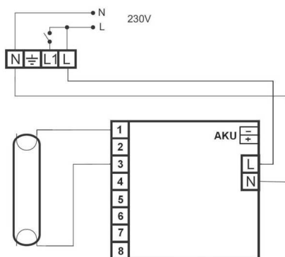
Emergency mode connection without ballast
