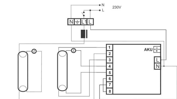
Connection to inductive ballast for fluorescent lamps arranged in serial layout
